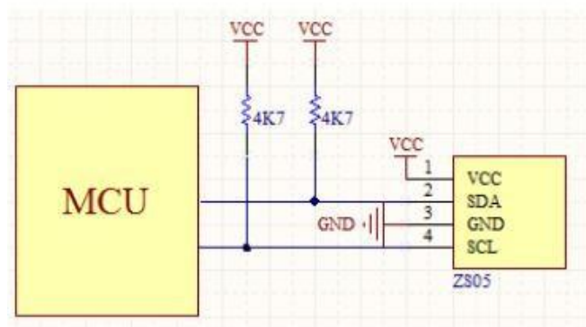
Fig3. application circuit
