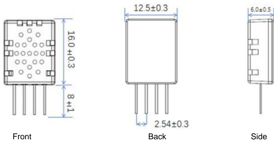
Fig1: Structure
