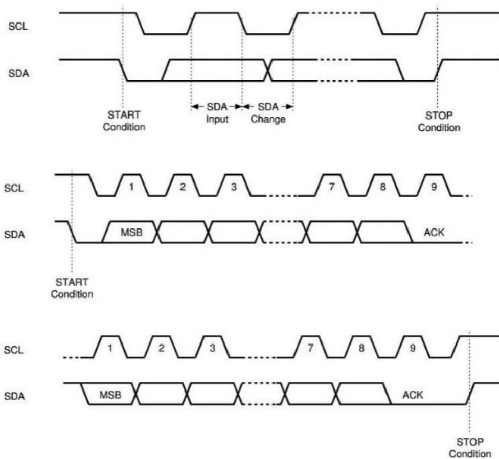
Fig4.IIC communication protocol
