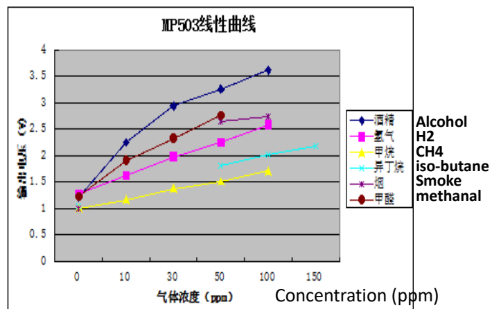
Fig6. Linearity curve
